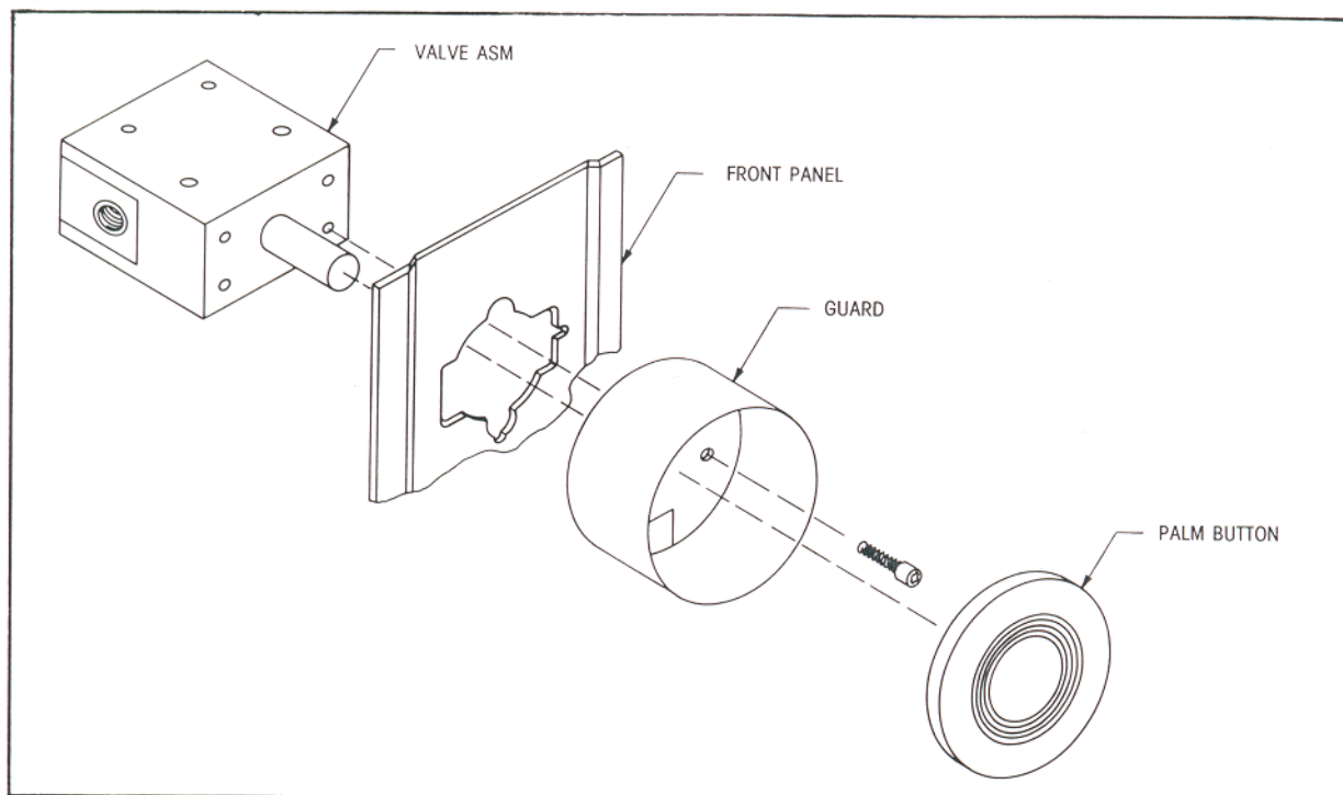
MODELS 460, 461 & 460, 461 W/29075 GUARD
