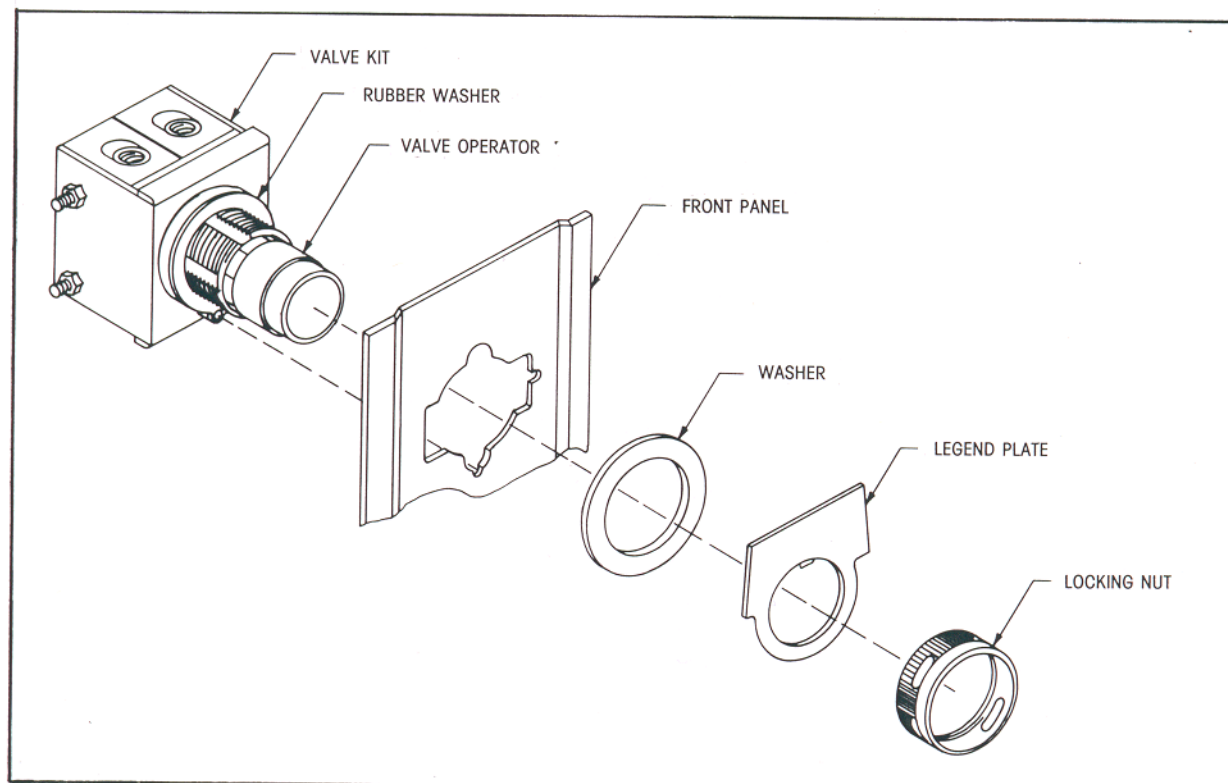
MODEL 59066X SWITCH & MODEL 59067 PUSH BUTTON
